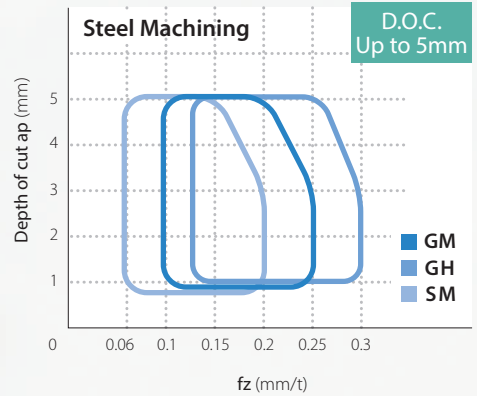
Applicable Chipbreaker Range
